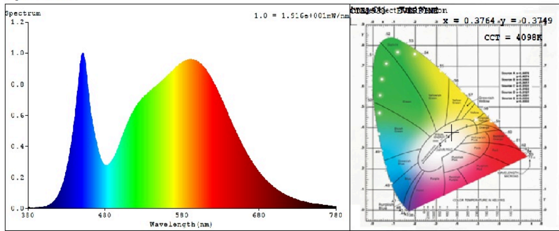
Spectral Distribution
